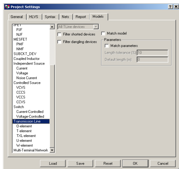
Figure 1. Specific SPICE elements.
