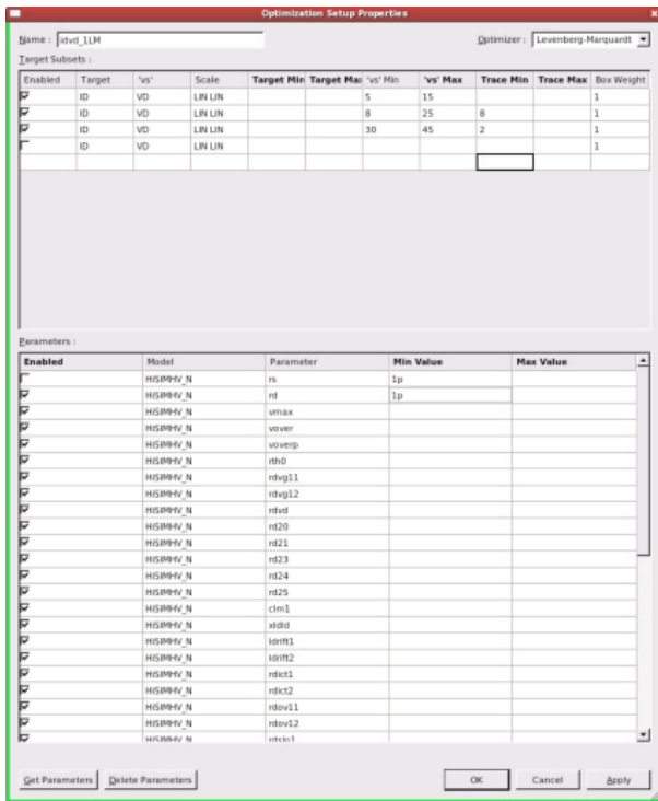
Figure-7 UTMOST-IV Optimization Setup Property for ids/vds.
