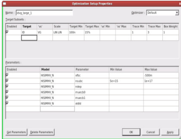
Figure-1 UTMOST-IV Optimization Setup Property for idvg_large_1.
