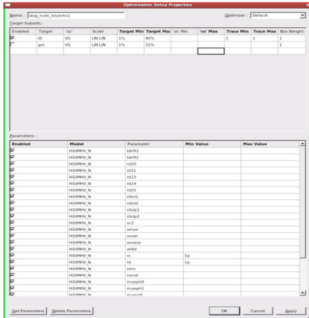
Figure-5 UTMOST-IV Optimization Setup Property for idvg_hvds_hisimhv1.
