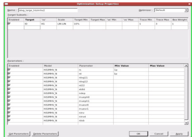
Figure-4 UTMOST-IV Optimization Setup Property for idvg_large_hisimhv2.
