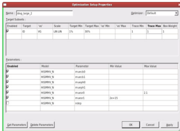
Figure-2 UTMOST-IV Optimization Setup Property for idvg_large_2 .
