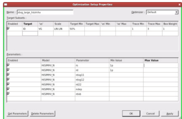
Figure-3 UTMOST-IV Optimization Setup Property for idvg_large_hisimhv.
