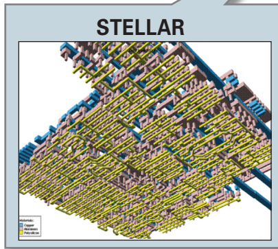
3D PHYSICS-BASED RC EXTRACTOR FOR LARGE CELLS
