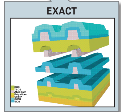
FULL CHIP LPE RULE FILE GENERATOR
