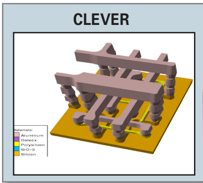
RC EXTRACTOR FOR REALISTIC 3D STRUCTURES
