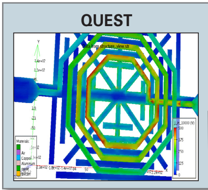
3D RF PASSIVE DEVICE MODELING
