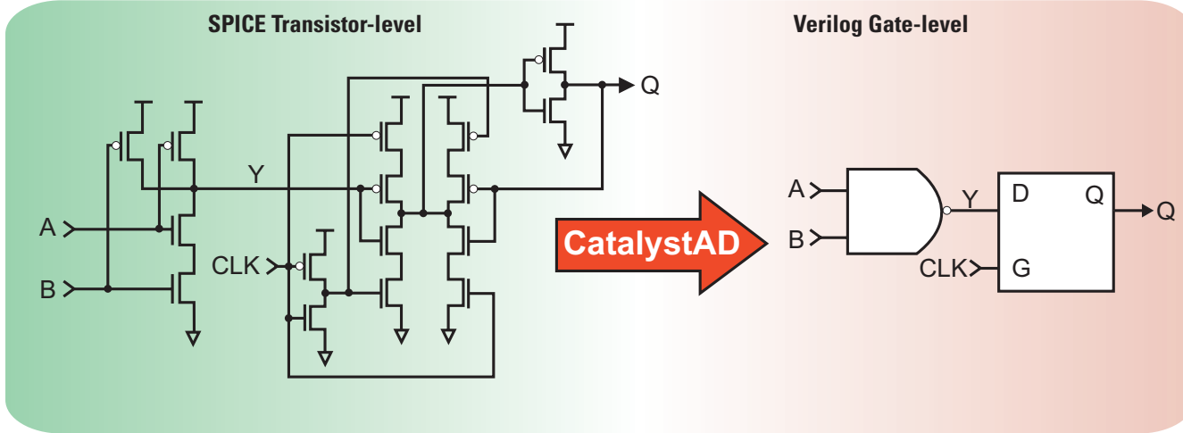
Automatic gate-level function extraction from a transistor-level netlist.
