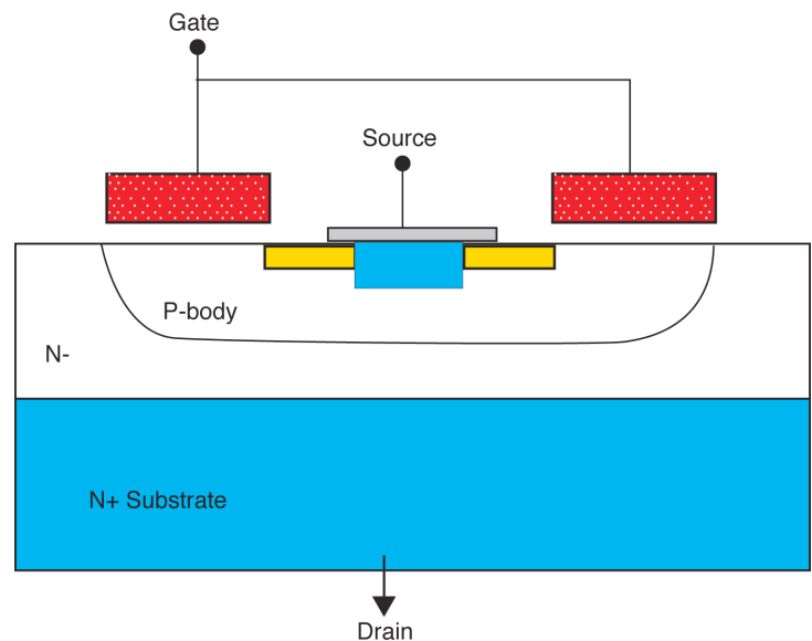
Schematic cross-section of a VDMOS device.
